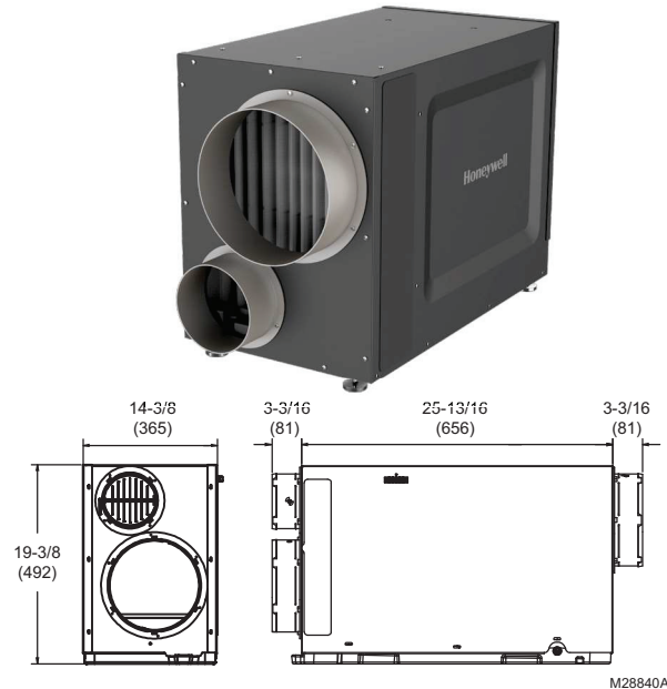
Fig. 1. Dimensions in in. (mm).
